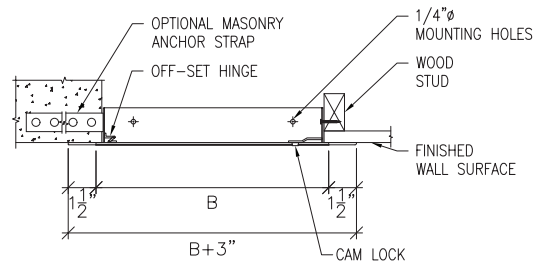
Section Detail
